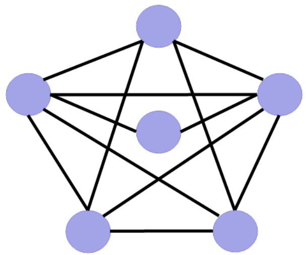
Not Hub-Centric Lt / Nt = 12/6 = 2.0 Lt / Lt Max = 12/15 = 0.80
